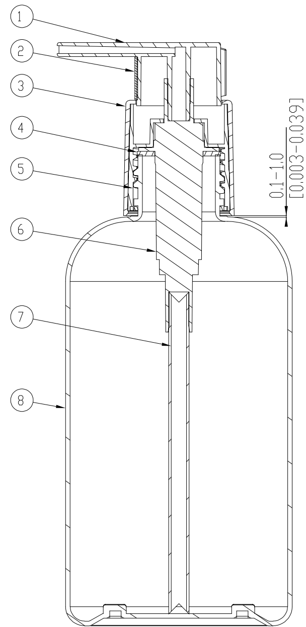
Section B-B
